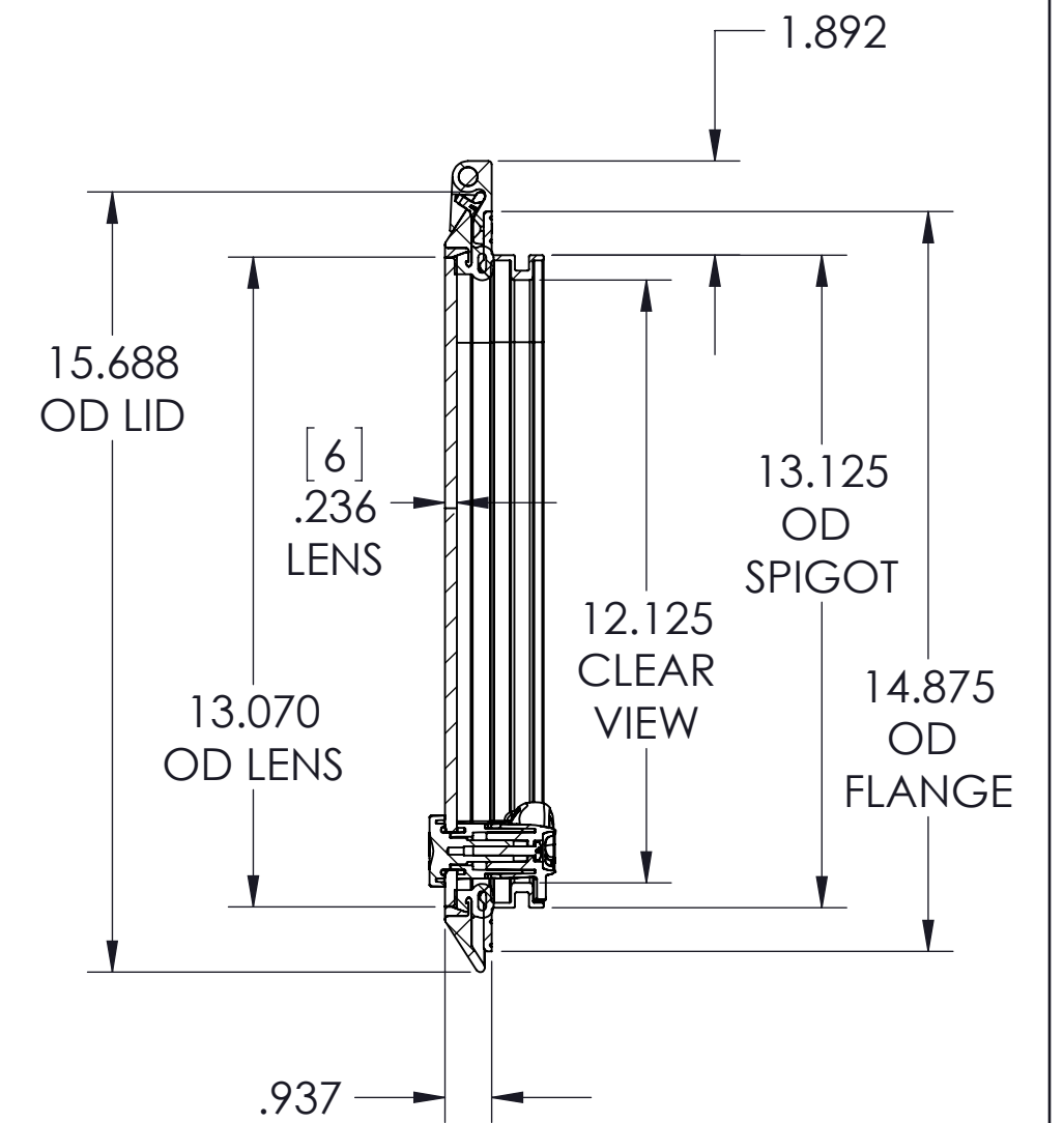
SECTION B-B
